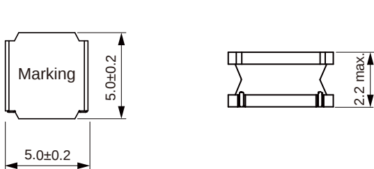
Dimensions: [mm]
