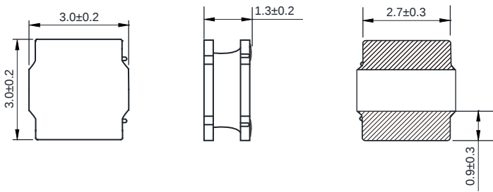
Dimensions: [mm]
