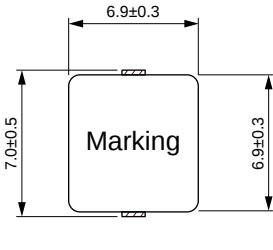
Dimensions: [mm]
