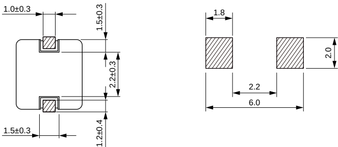
Land Pattern: [mm]
